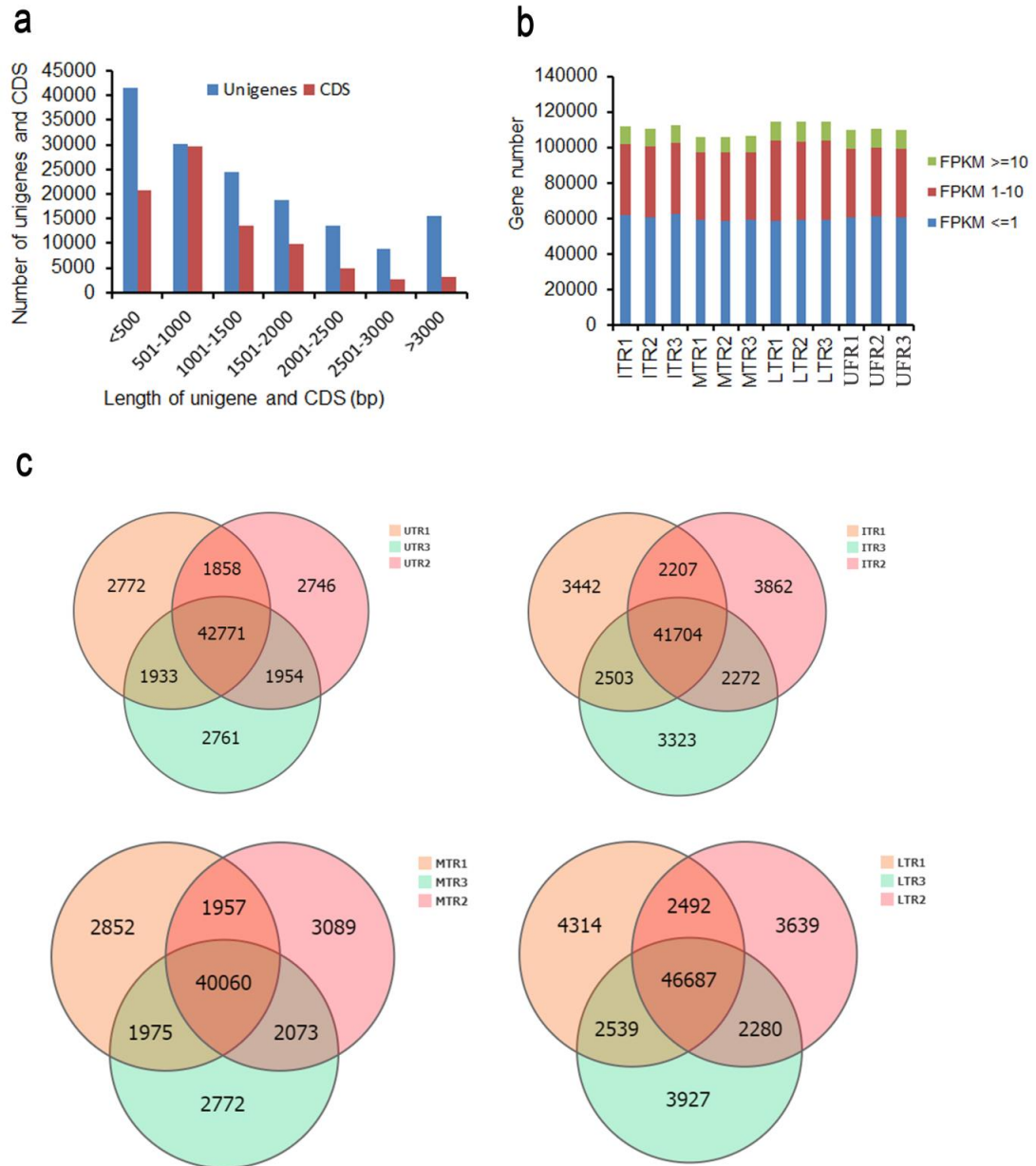
Fig. S1. Distribution and Venn diagram analysis of transcripts. a. Length distribution of the assembled unigenes and CDSs. b. Gene expression distribution of each sample. c. Venn diagram analysis among three different samples at the same development stage.
